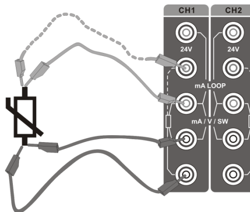
Figure 4 NTC Connection
